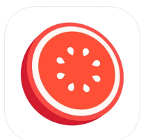
Focus Keeper
